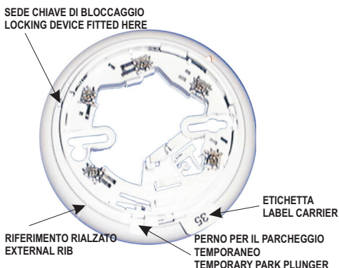
FIG. 2 Base Universale 5B 5B Universal Base
